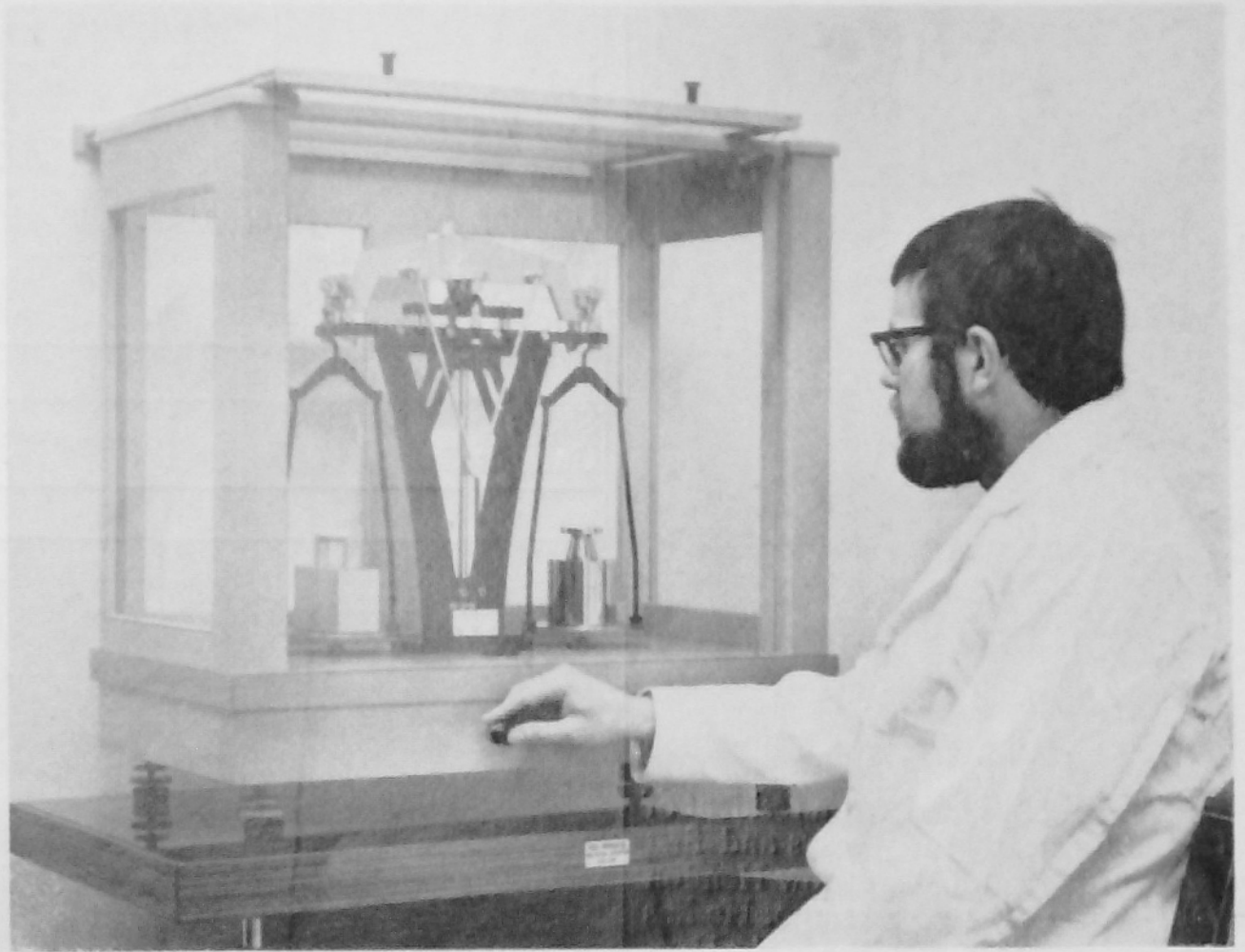
An Inspector compares Working Standard weight with the Local Standard.
