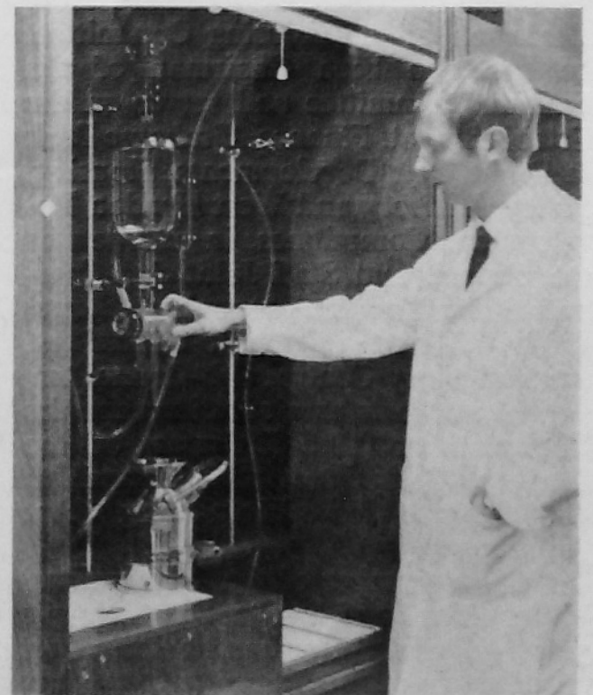
Working Standard "Chekpump" measure being calibrated against the Local Standard.
